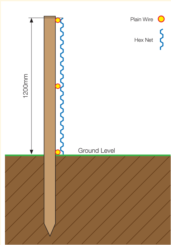
Fence Configuration Detail
